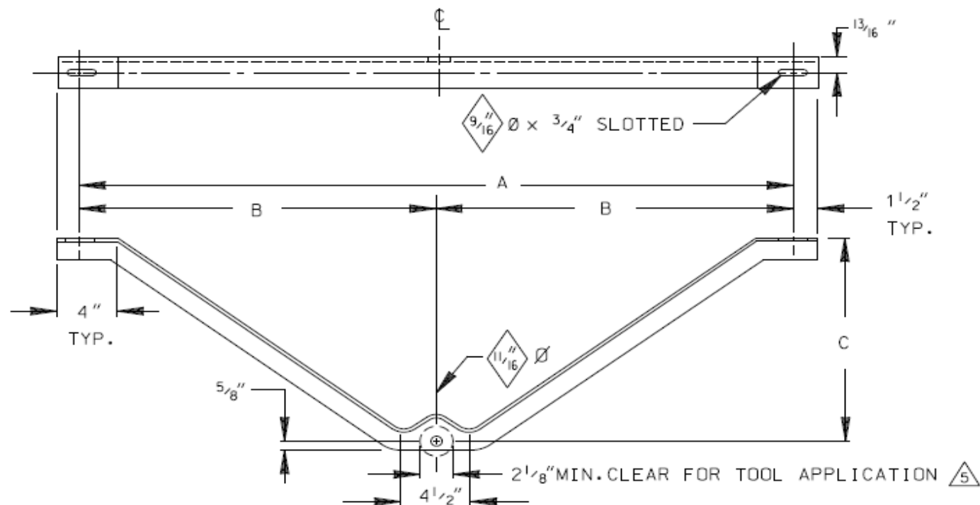
ANGLE BRACE
